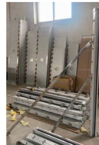
2 or 3 pcs of support braces can be applied on high center post.
