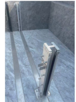
304 stainless steel base plate under aluminum flood barrier.
